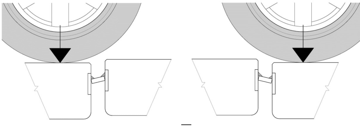
Figure 2 Exaggerated depiction of beam deflection at flange joint connection.
