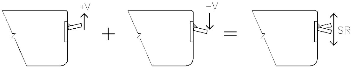
Figure 22 Stress Range pictorial.
