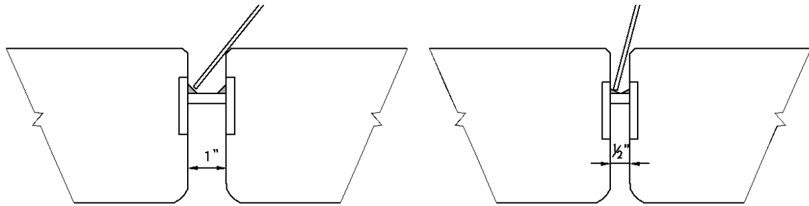
Figure 37 Weld angle for varying joint widths.
