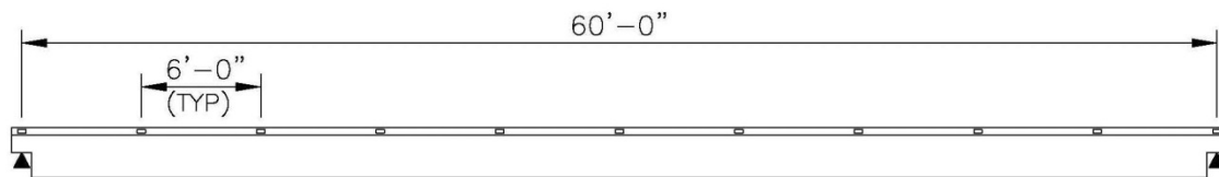
Figure 18 Beam elevation.
