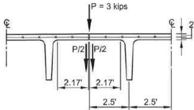
Figure 12 Excerpt from Example 5.12.1.1, Flexural Strength of Double-Tee Flange in Transverse Direction. Credit: Precast/Prestressed Concrete Institute, Force, Greg, et al, PCI Design Handbook, 7 th ed., 2010.
