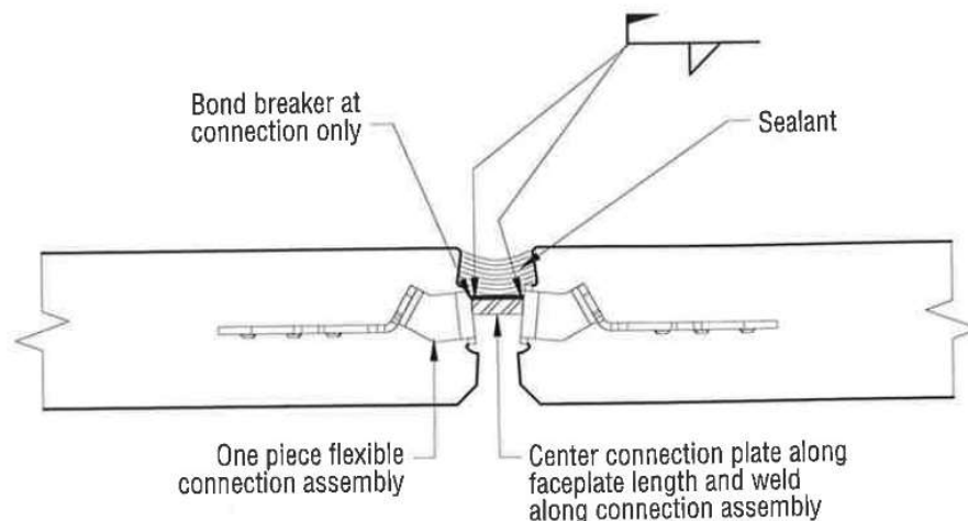
Figure 3-7 Pretopped Flange Connector
