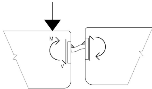
Figure 20 Shear and bending forces on welded connection.
