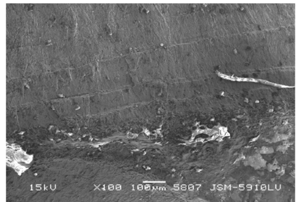
Figure 11B Fatigue failure of a flat bar-type connection; scanning electron micrograph.
