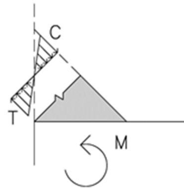
Figure 24 Internal stress at throat of weld.
