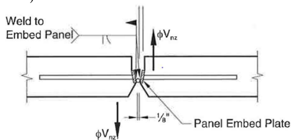
– Figure 13 Excerpts from Example 3.12, Double-Tee Flange to Flange. Precast/Prestressed Concrete Institute, Sennour, Larbi et al, PCI Connections Manual for precast and prestressed concrete construction, 1 st ed., 2008.
